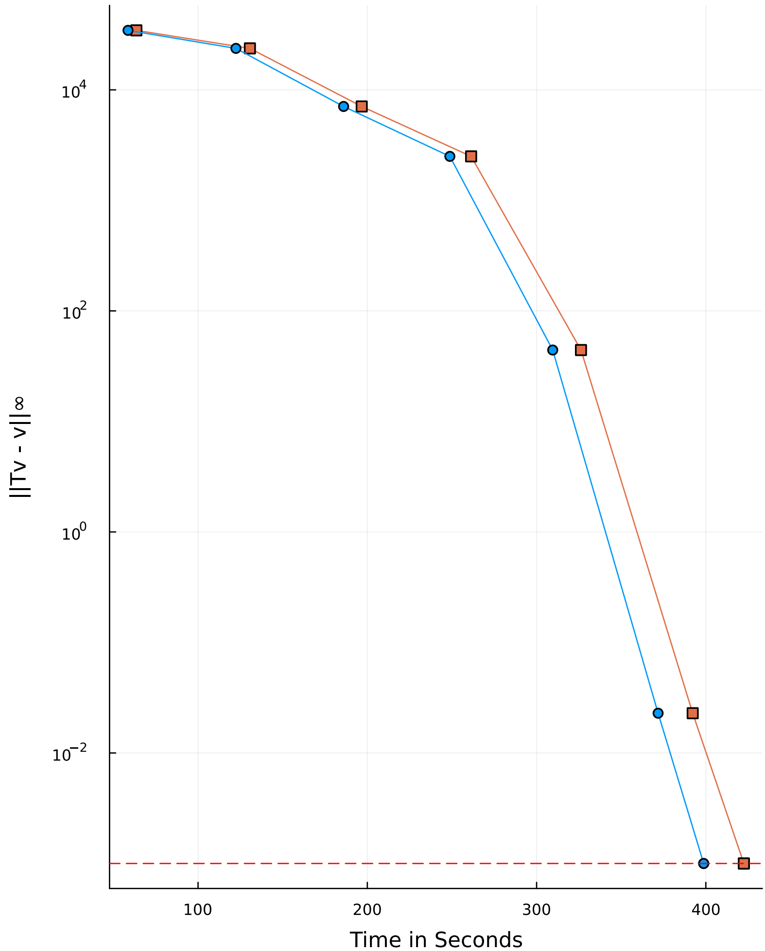
Large Problems
